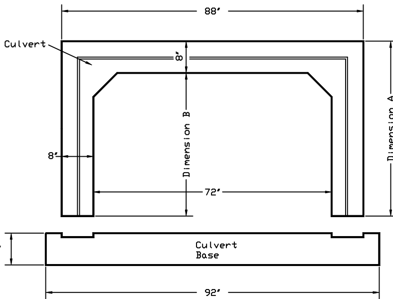
END VIEW
