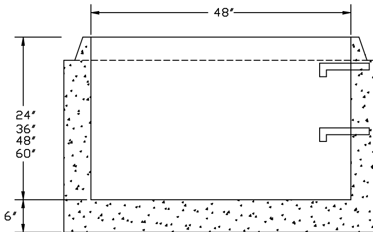
48" MONOBASE
