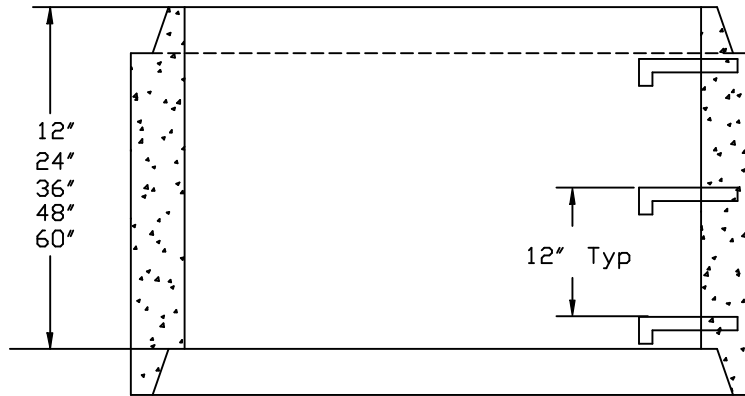
48" RISER SECTION
