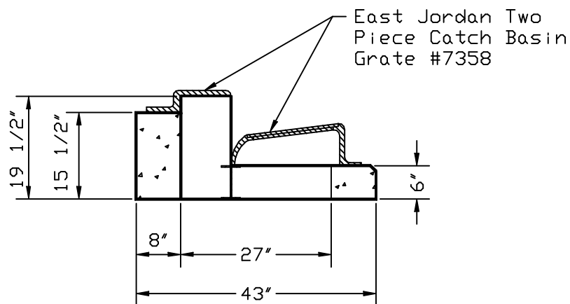
SECTION END VIEW
