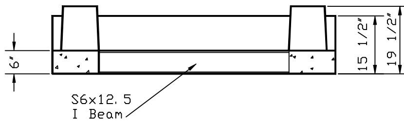
FRONT VIEW SECTION
