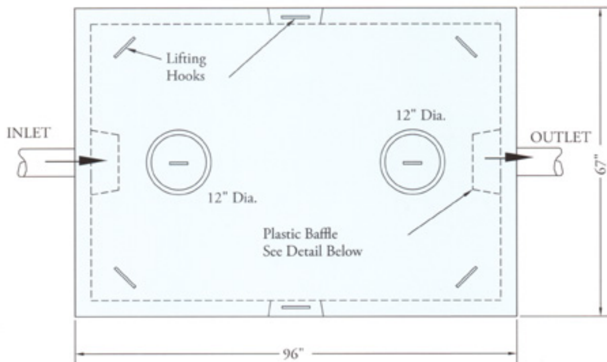
TOP VIEW
